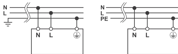
AC Line
