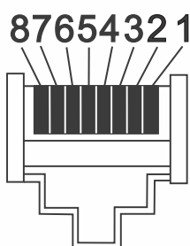
RJ45 male
