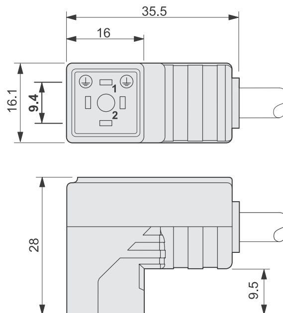
Valve connector type CI
