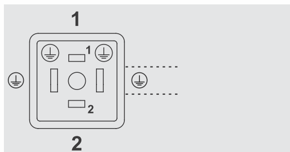
Valve connector type CI
