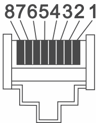
RJ45 male
