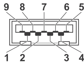
USB 3.0 A female
