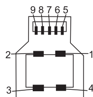
USB 3.0 B female
