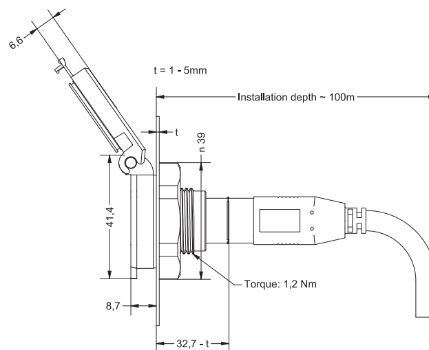
USB 3.0 B female
