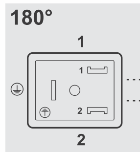
Valve connector type B
